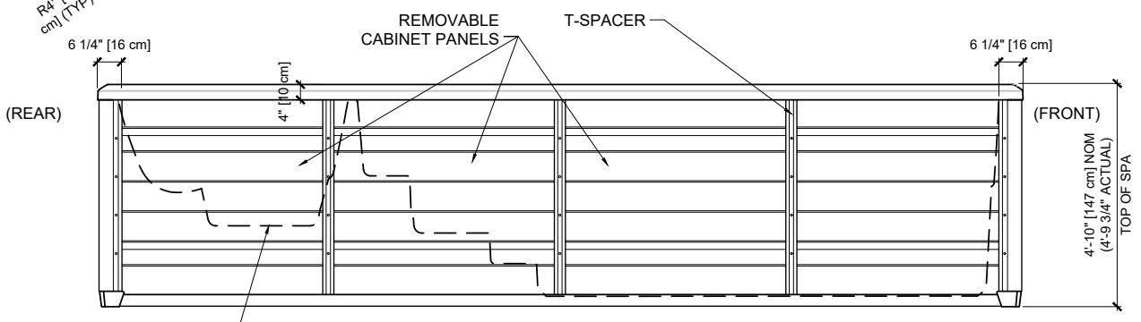
OUTLINE OF SHELL RIGHT ELEVATION
